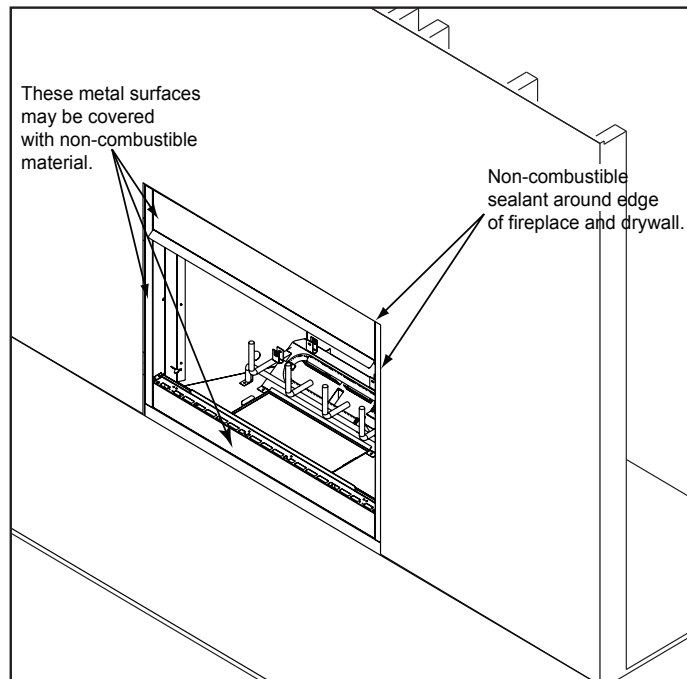
Figure 7.1 Noncombustible Facing
