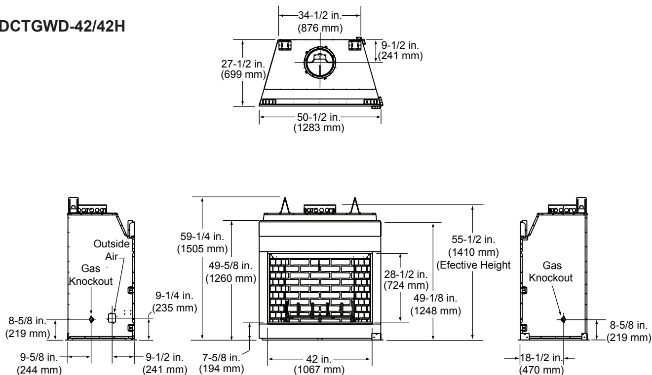
Figure 3.1 Fireplace Dimensions
