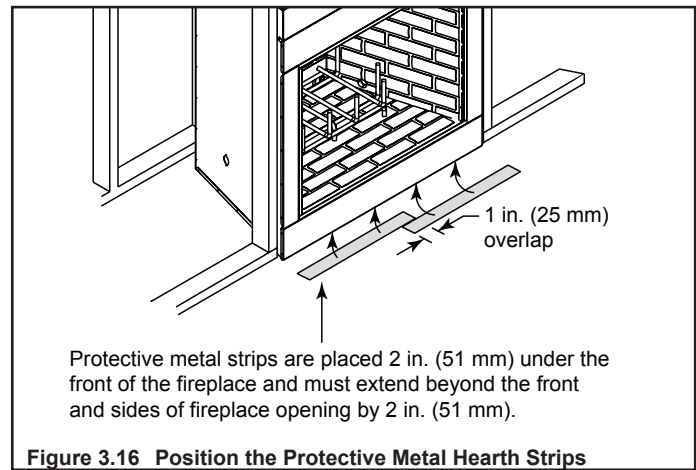
Figure 3.16 Position the Protective Metal Hearth Strips
