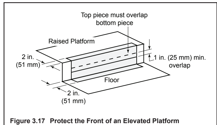
Figure 3.17 Protect the Front of an Elevated Platform
