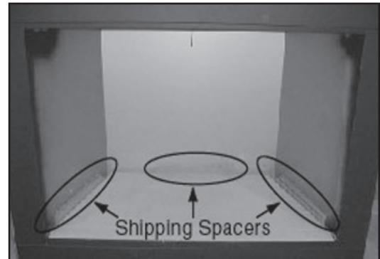
Figure 3.10 Shipping Spacers
